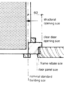
⑥ Recessed door frame
